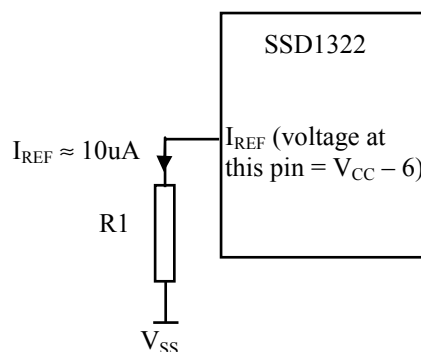
Figure 8-8 : I Current Setting by Resistor Value
