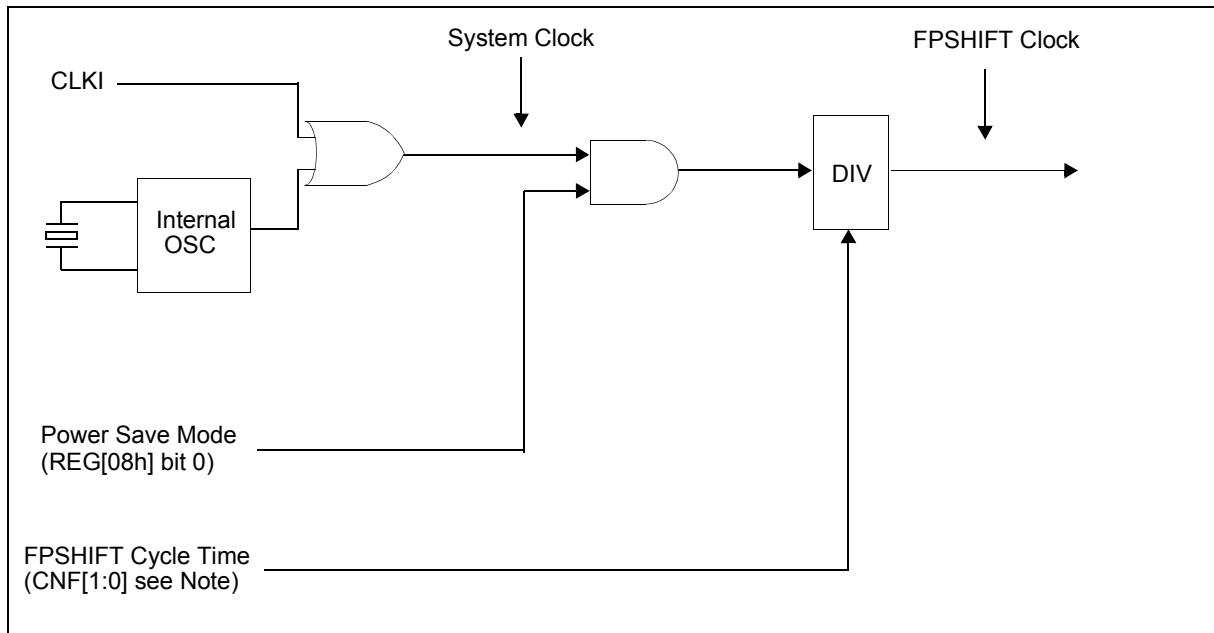
Figure 9-1: Clock Diagram
