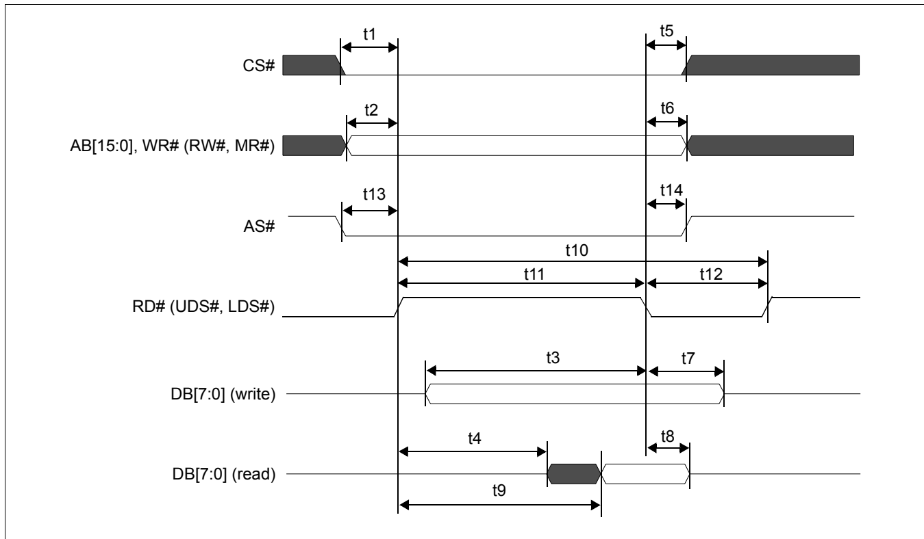
Figure 7-7 M6800 Family Bus Indirect Interface Timing
