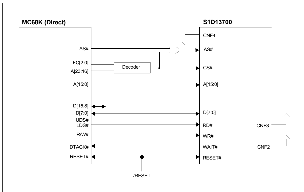
Figure 3-4 Direct MC68K to S1D13700 Interface Example
