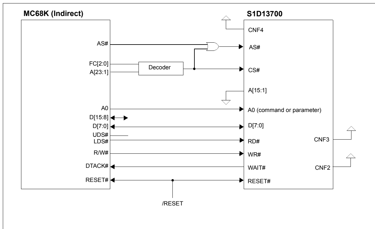
Figure 3-3 Indirect MC68K to S1D13700 Interface Example
