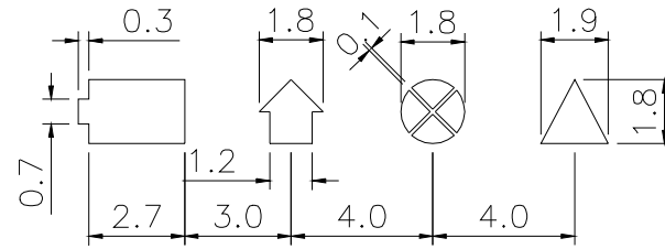
Detail B
