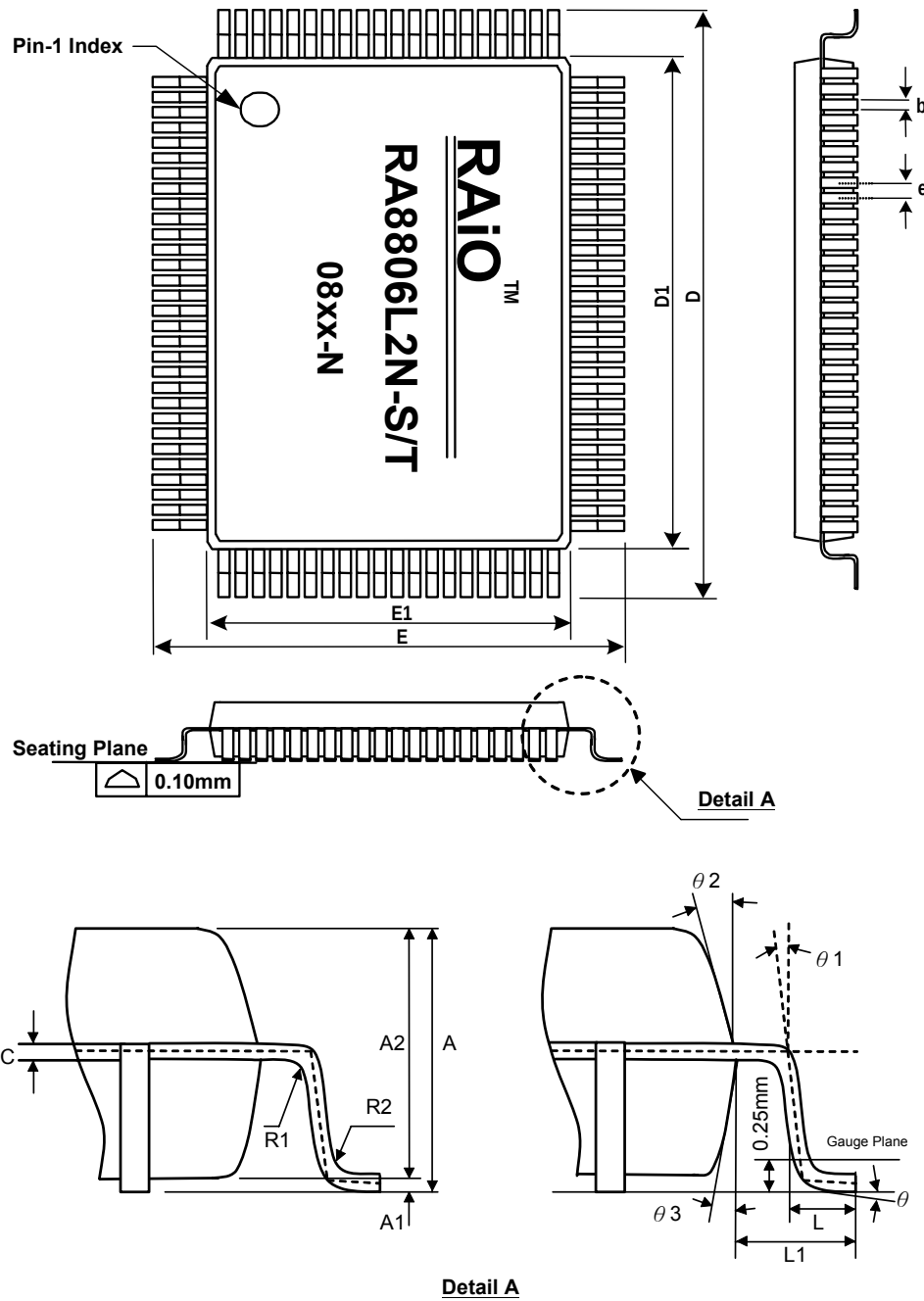
Figure 7-4 : LQFP-100Pin Mechanical
