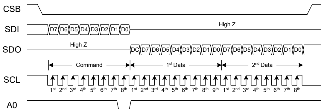
Figure 7 Read-Operation of 4-Line Serial Interface
