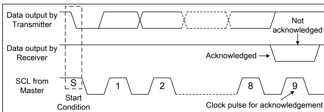
Figure 13 Acknowledgement of I 2 C Interface
