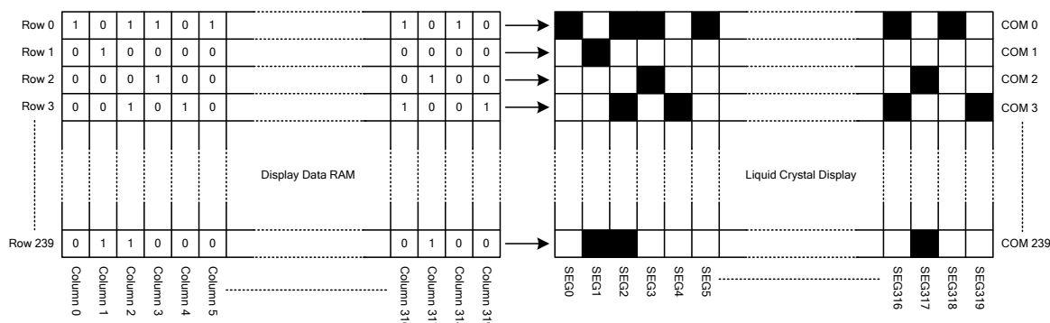
Figure 15 DDRAM Mapping
