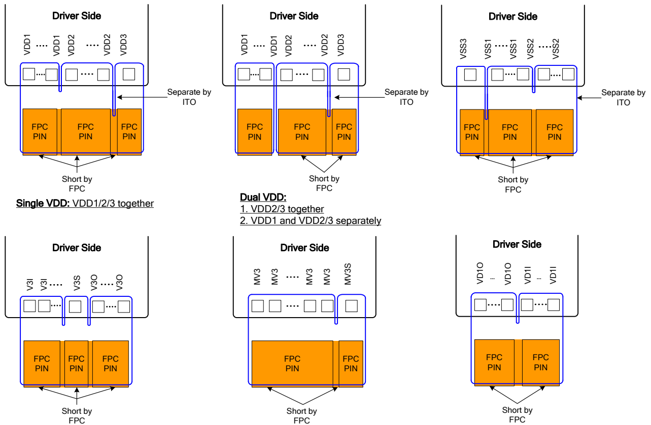
Figure 3 Power Pin ITO Layout
