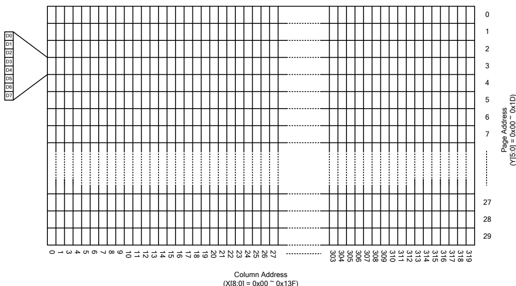
Figure 16 DDRAM Format
