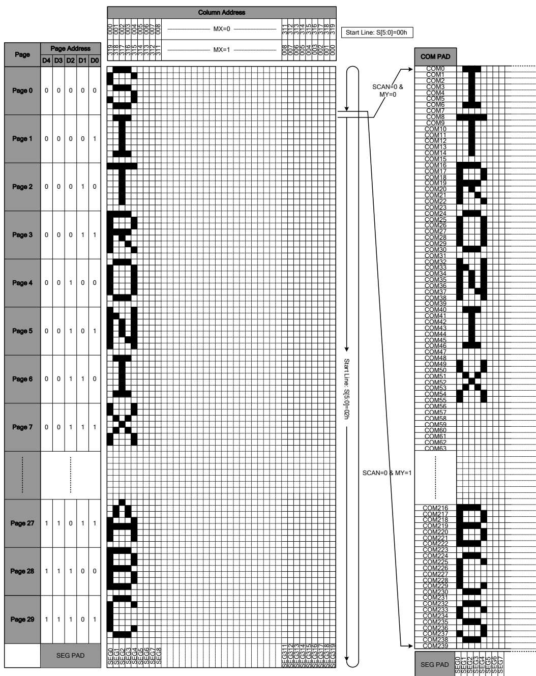
Figure 18 Display Data RAM Map (1/240 Duty)
