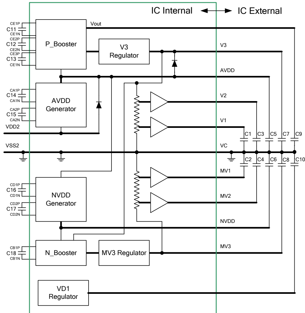
Figure 19 Internal Power Circuits & External Connection
