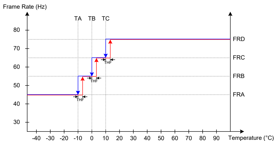
Figure 23 Frame Rate
