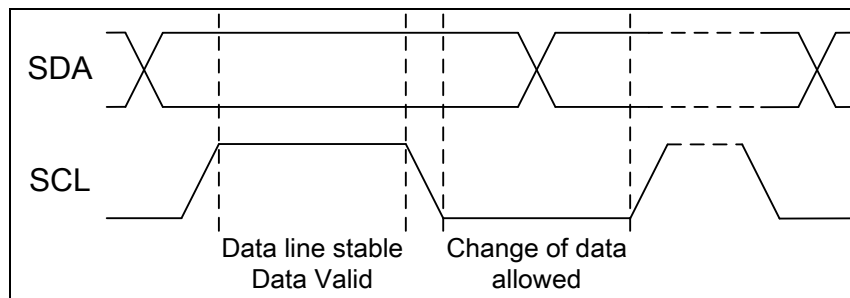
Figure 10 Bit Transfer
