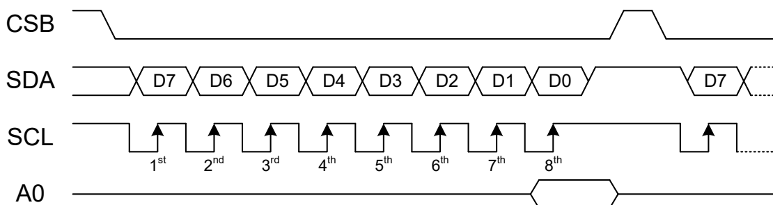
Figure 6 Write-Operation of 4-Line Serial Interface
