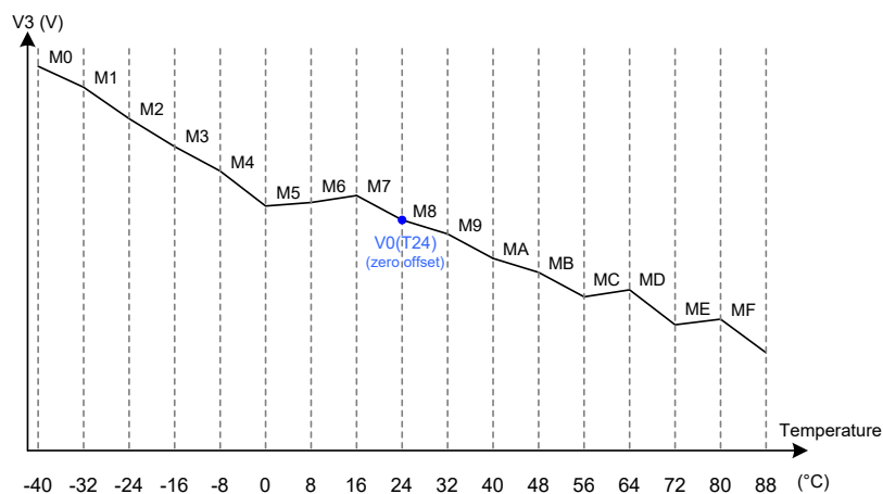
Figure 22 Temperature Gradient Compensation
