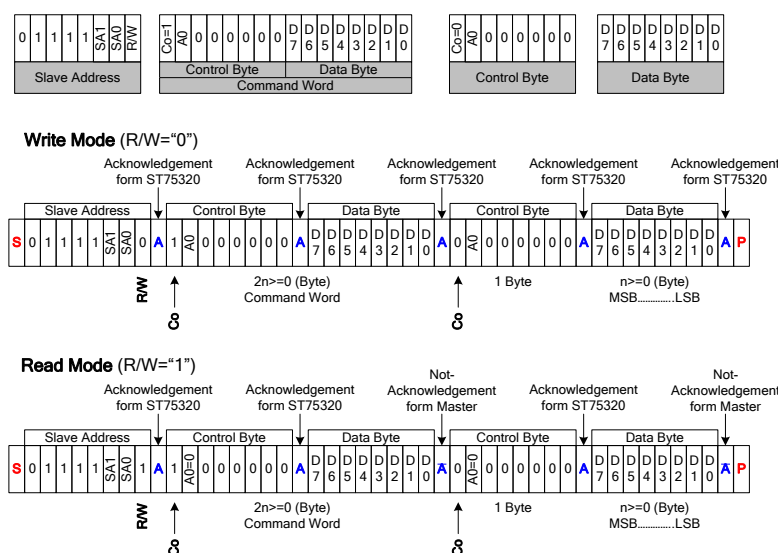
Figure 14 I 2 C Interface Protocol
