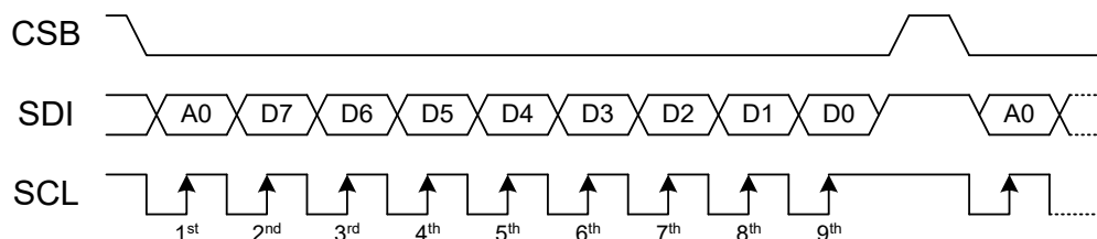
Figure 8 Write-Operation of 3-Line Serial Interface
