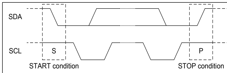
Figure 11 Definition of START and STOP Condition
