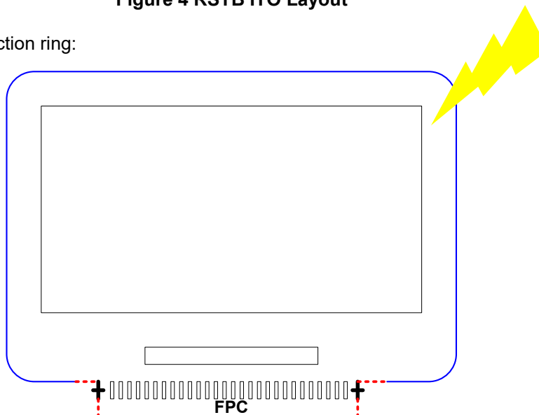
Figure 4 RSTB ITO Layout
