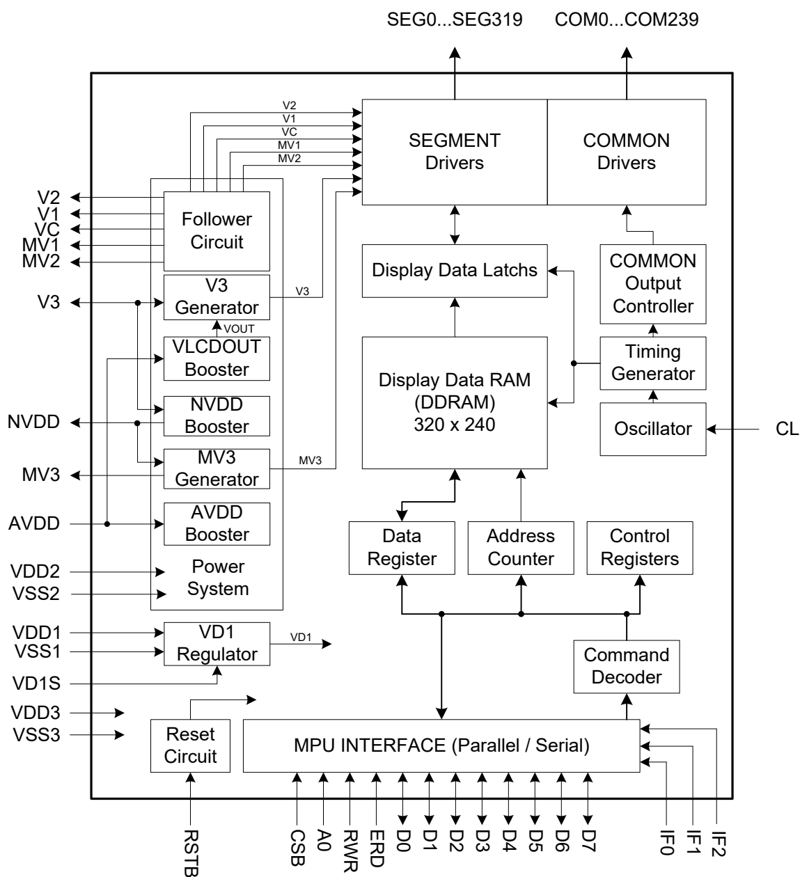
Figure 2 Block Diagram
