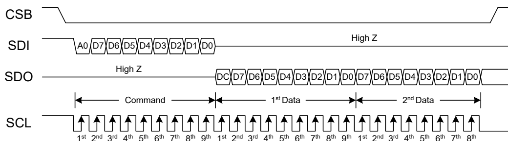
Figure 9 Read-Operation of 3-Line Serial Interface
