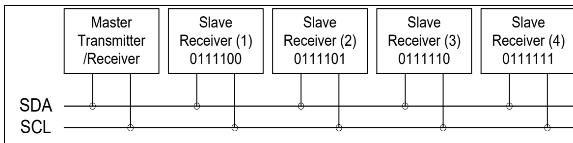
Figure 12 System Configuration
