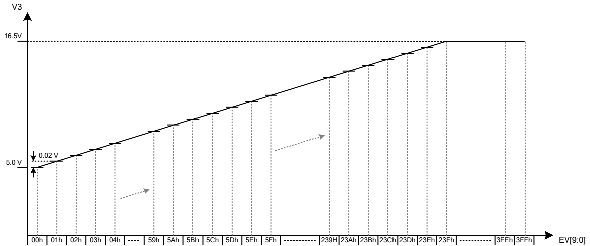
Figure 20 Vop Programmable Range
