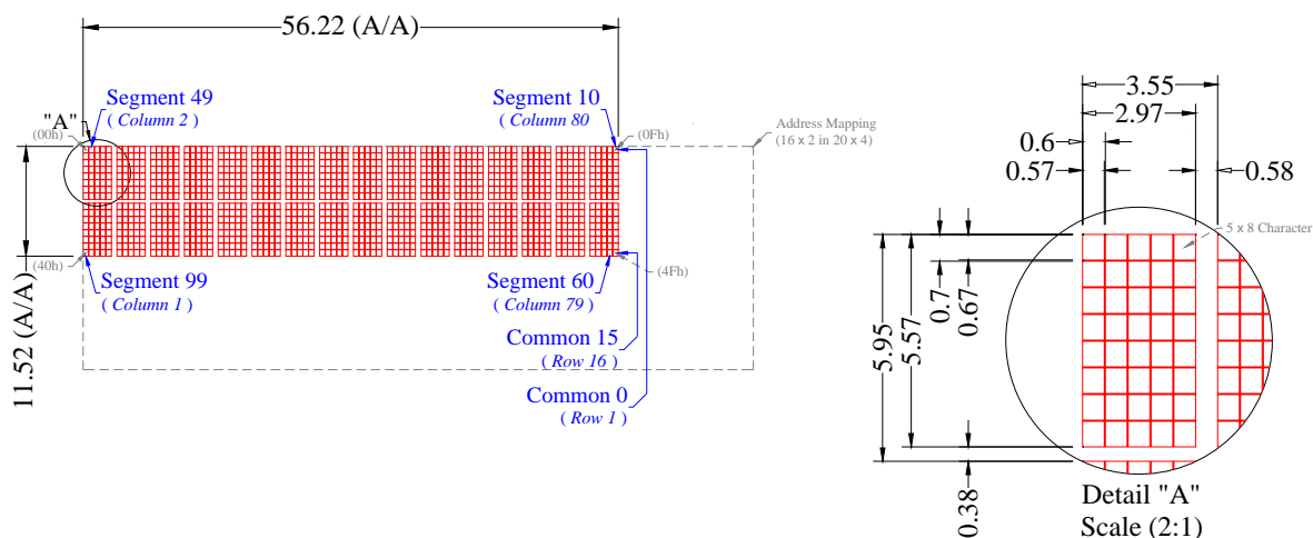
Address Mapping
