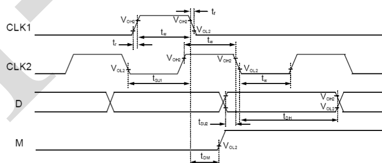
Figure 3 . Interface Mode with Extension Driver
