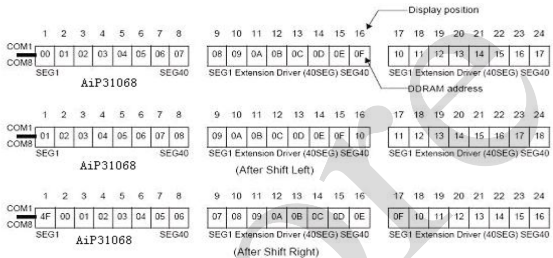
Figure 5 . 1-line × 24 char. display with 40 SEG. extension driver
