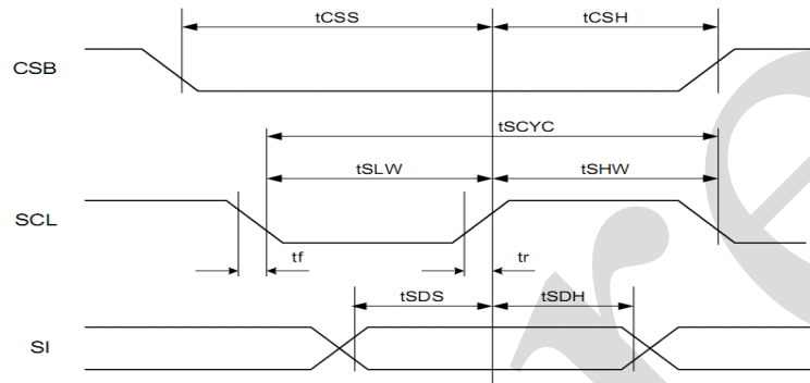
Figure 1 . Timing Diagram of 3-lines interface
