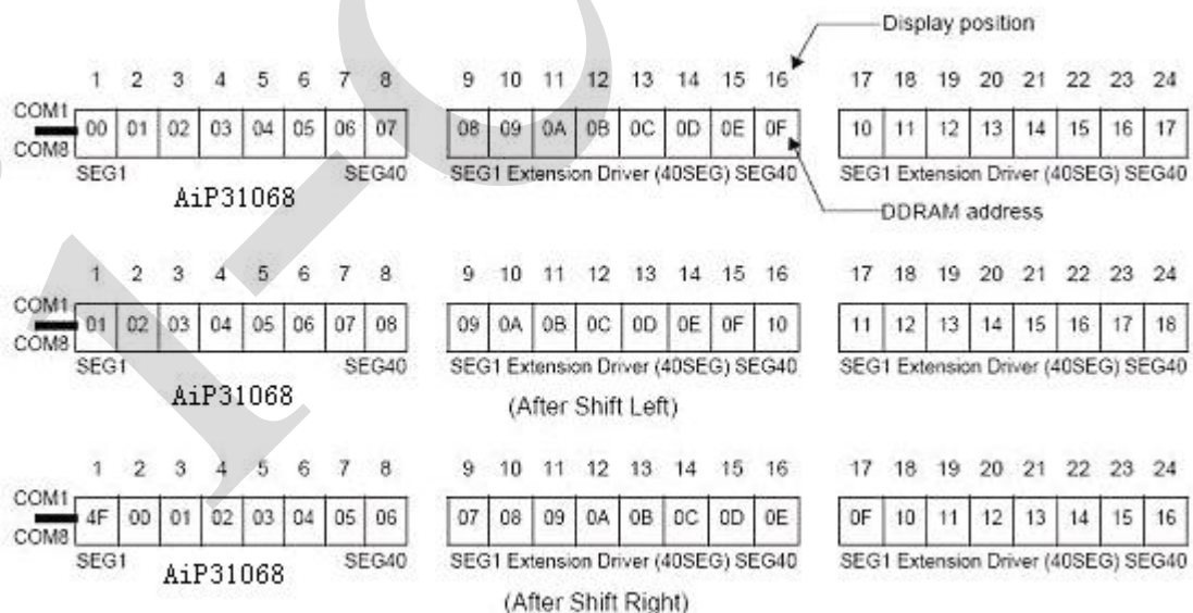
Figure 6 . 2-line × 24 char. display with 40 SEG. extension driver
