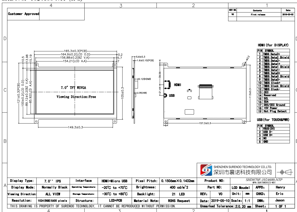
SHD070F-1024600-NTP (IPS)
